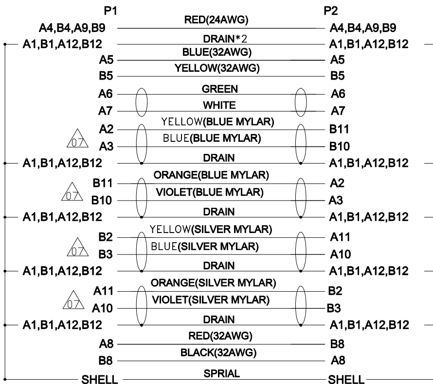
Wiring Diagram
