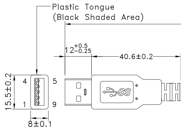
USB3.0 A MALE MOLDED BLACK (P1)
