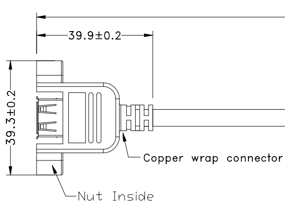
USB A 3.0 FEMALE MOLDED BLACK
