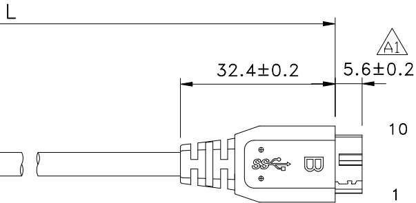
Micro-USB 3.0 BM MOLDED BLACK
